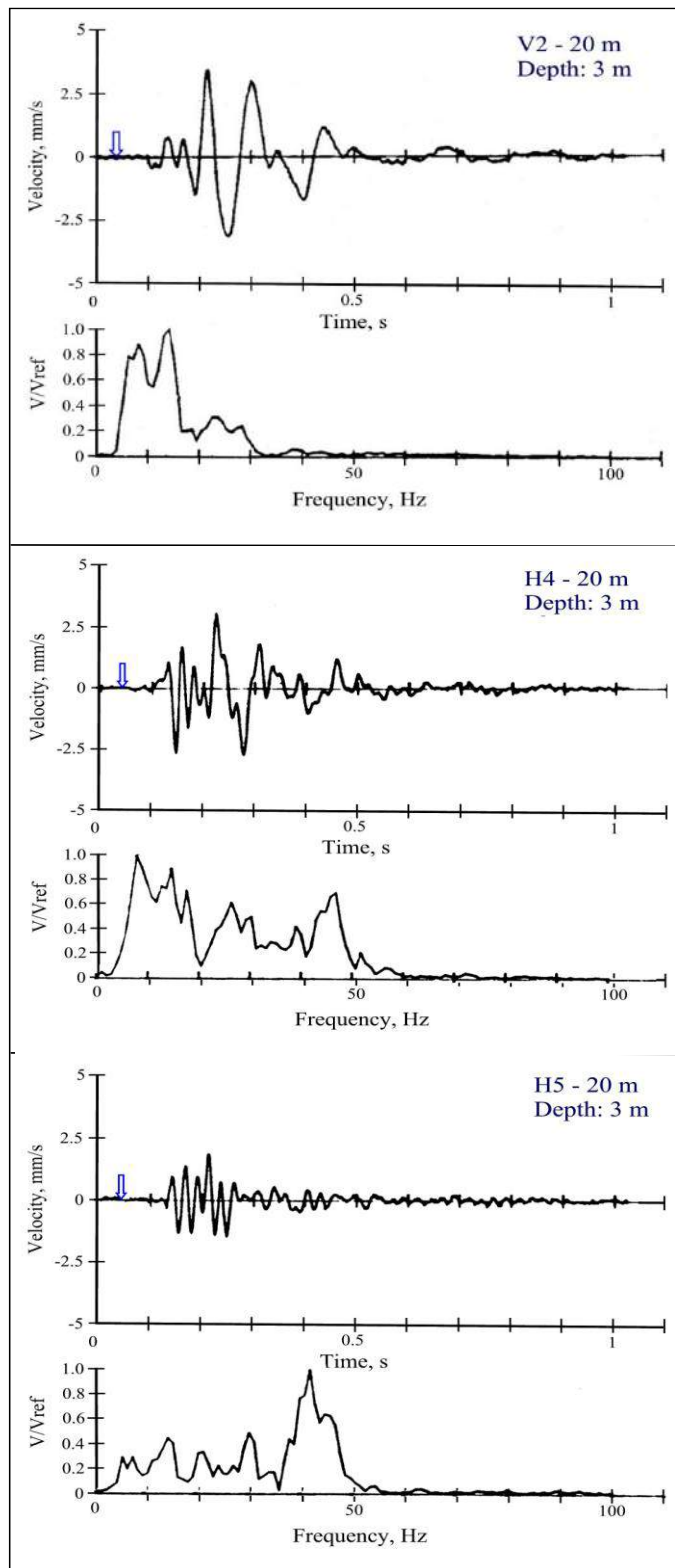
Fig. 21. Vibration velocity records and normalized Fourier spectra at 20 m distance for sensors V2 (vertical), H4 (radial) and H5 (transversal) during pile driving at 3 m depth. The arrow indicates the instant of hammer impact.
