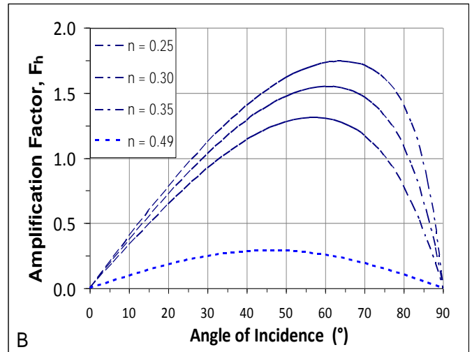
Fig. 13. Variation of vibration amplification factors, F_v and F_h , at the free surface of an impinging P-wave for different values of Poisson's ratio.
