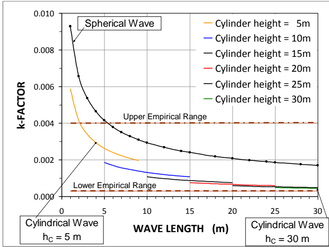
Fig. 12. Variation of k-factor (Eq. 3) as function of wave length according to Table 9 for a spherical wave and cylinder waves with height ranging from 5 m through 30 m. Soil density is 1,800 kg/m 3 . Upper and Lower Empirical Range according to Fig. 4.
