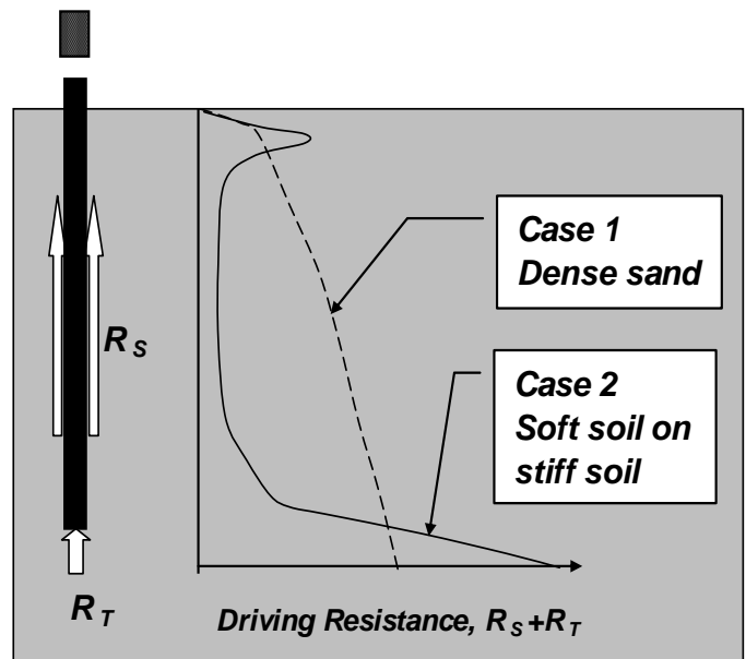
Fig. 6. Conceptual picture of soil resistance along the shaft, R_S and toe, R_T when driving a pile into dense sand and soft clay on a stiff layer, respectively. Note, the driving resistance is indicated in units of force, not in units of penetration resistance ("blow count").
