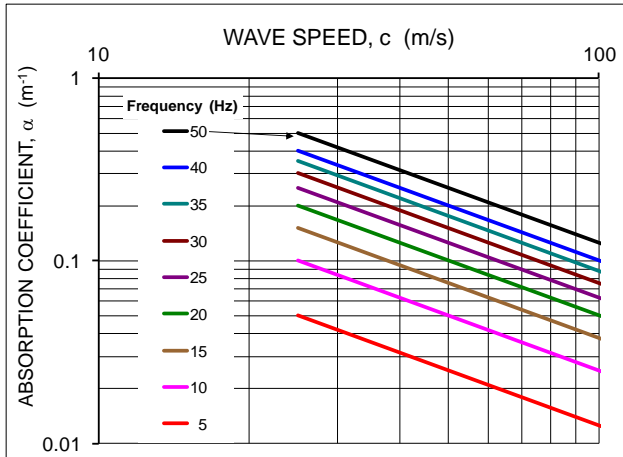
Fig. 15. Absorption coefficient \alpha as function of wave speed for different vibration frequencies (the assumed value of material damping is 4 %).
