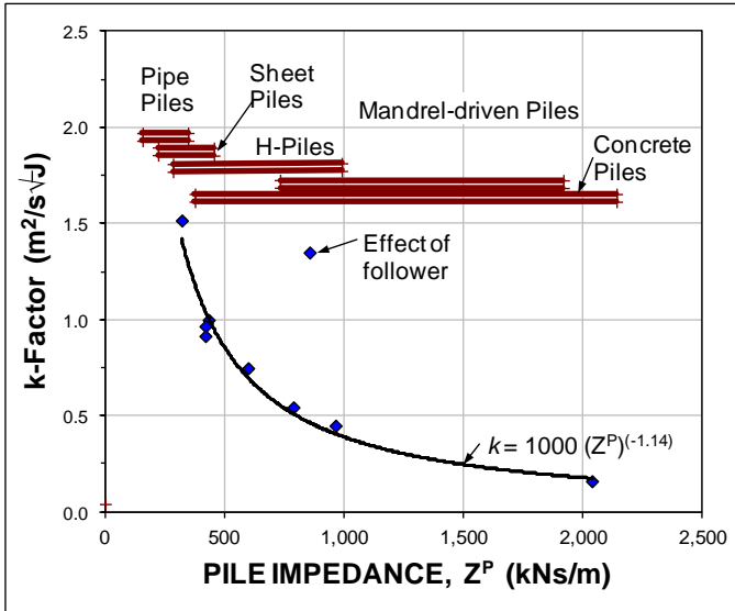
Fig. 10a. Influence of pile impedance on the vibration factor, k (Eq. 3). (Data from Heckman and Hagerty 1978).
