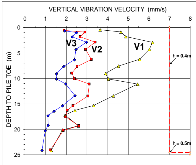
Fig. 19. Vertical vibration velocity at three distances as function of pile depth together with the hammer height-of-fall.
