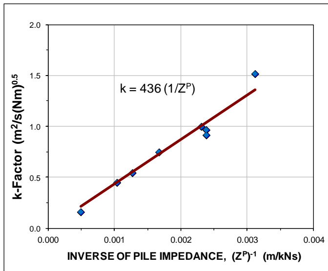
Fig. 10b. Relationship between k -factor and inverse of pile impedance, data from Fig. 10a replotted.
