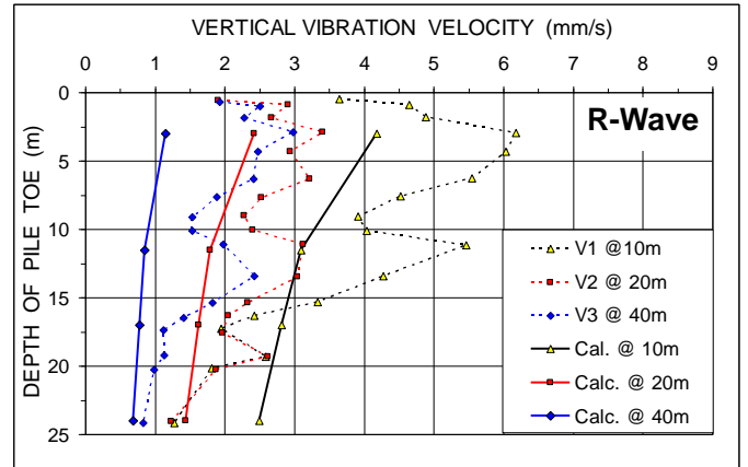
Fig. 27. Vertical vibration velocities (dashed lines) measured at 10, 20, and 40 m distance from the pile and calculated (solid lines) speeds caused by surface waves (R-waves) emitted from pile toe and refracted at the surface.
