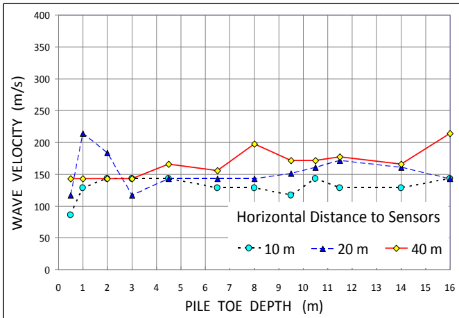
Fig. 24. Speed of cylindrical wave, determined from first peak of speed amplitude at sensors V1, V2, and V3, respectively, as measured at different pile toe depths.
