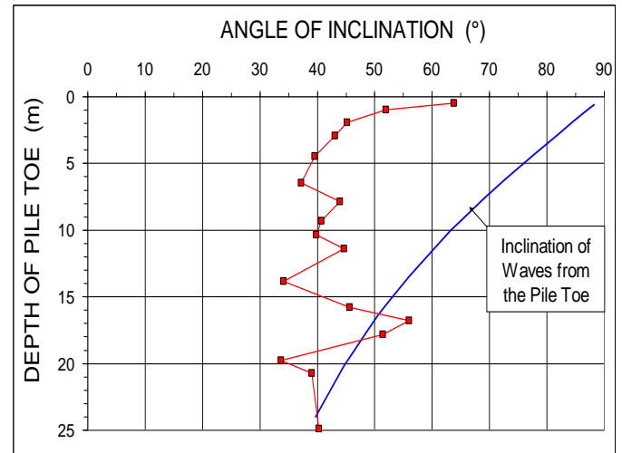
Fig. 18. Inclination of resultant vibration amplitude (as angle to the vertical) and estimated angle of incidence of waves emitted from pile toe. Note that a low angle of inclination implies a larger vertical vibration amplitude.
