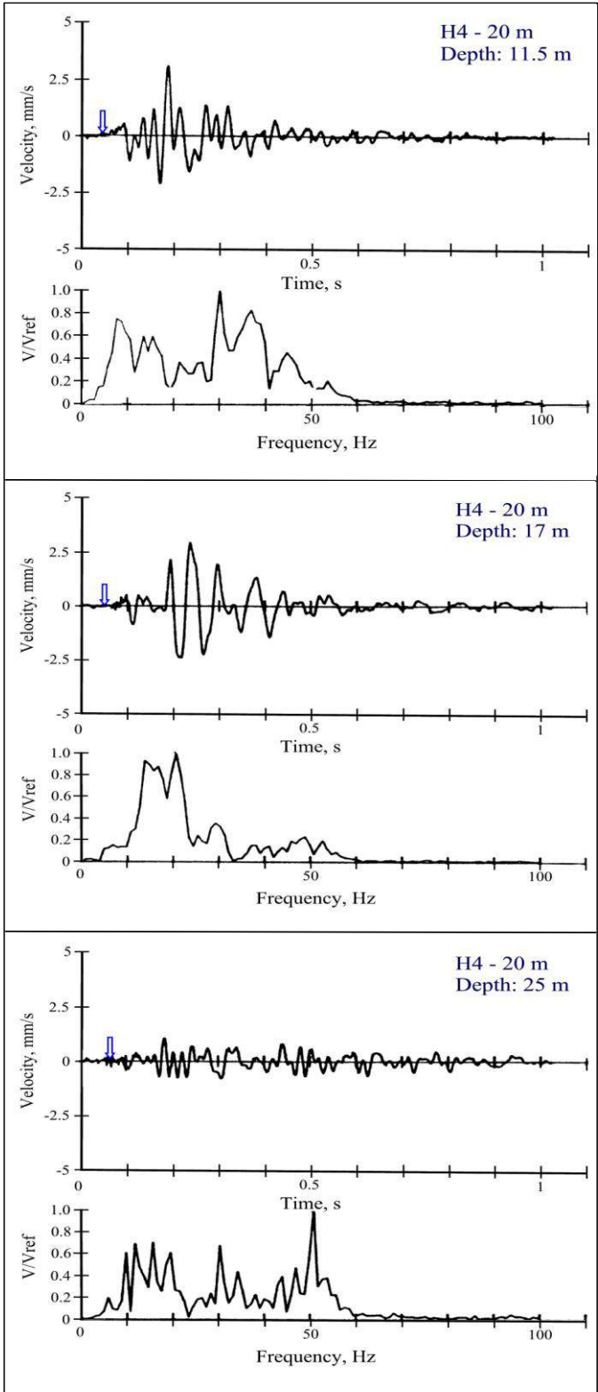
Fig. 23. Vertical vibration velocity records and normalized Fourier spectra for measurement location H4 (radial), during pile driving at 11.5, 17, and 25 m depth. The arrow indicates the time of hammer impact.
