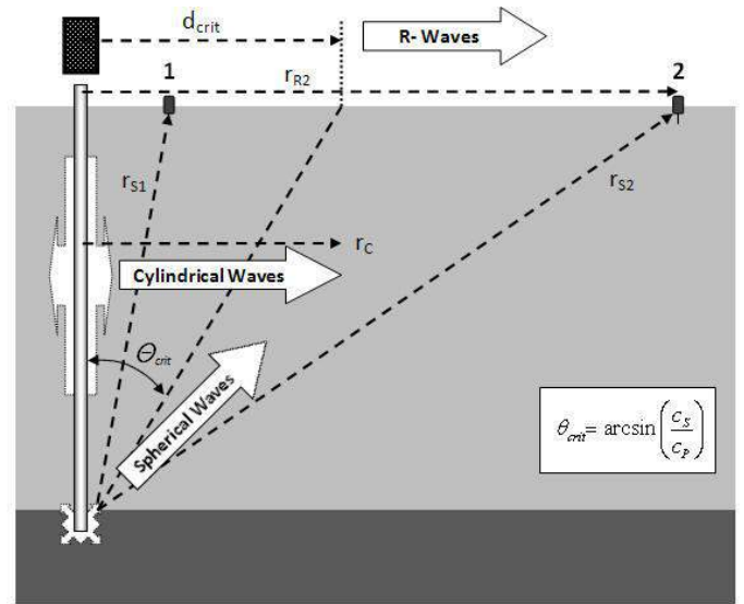
Fig. 11. Illustration of vibrations emitted during pile driving at the pile toe and along the pile shaft; c_s = shear wave speed in the soil; c_p = stress wave speed in the soil. d_{crit} = critical distance from pile.
