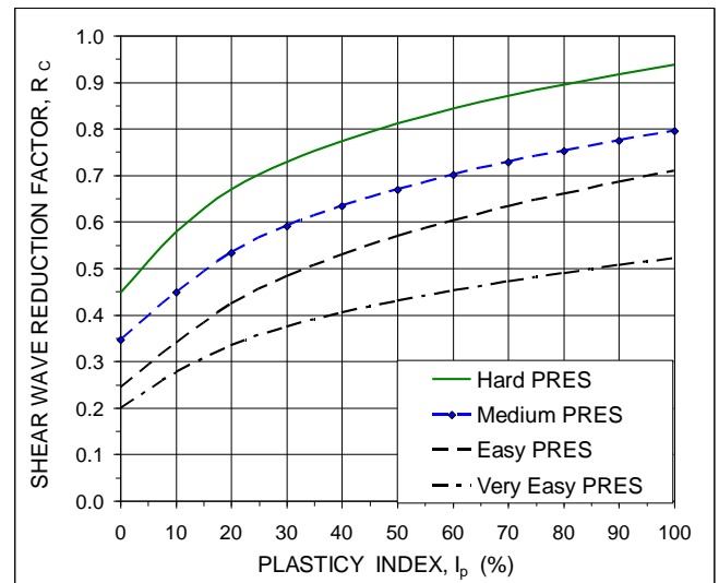
Fig. 8. Shear wave speed reduction factor, R_C as function of plasticity index, I_p , for different conditions of penetration resistance, PRES, modified from Massarsch (2005).
