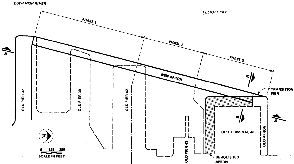
Figure 1. Site plan, Southeast Harbor Development Project.
