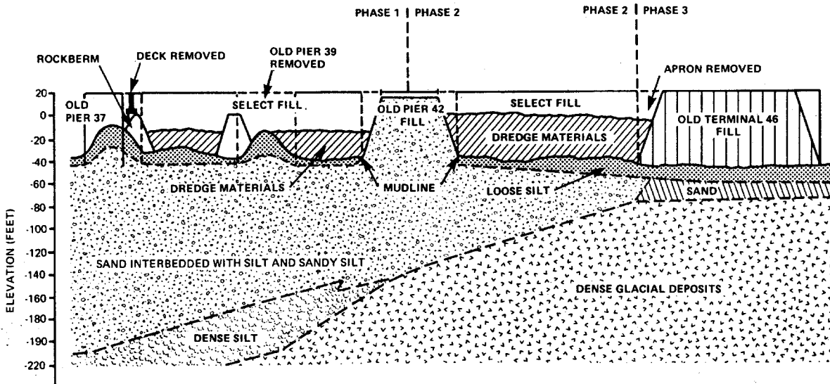
Figure 2. Section A-A of Figure 1.
