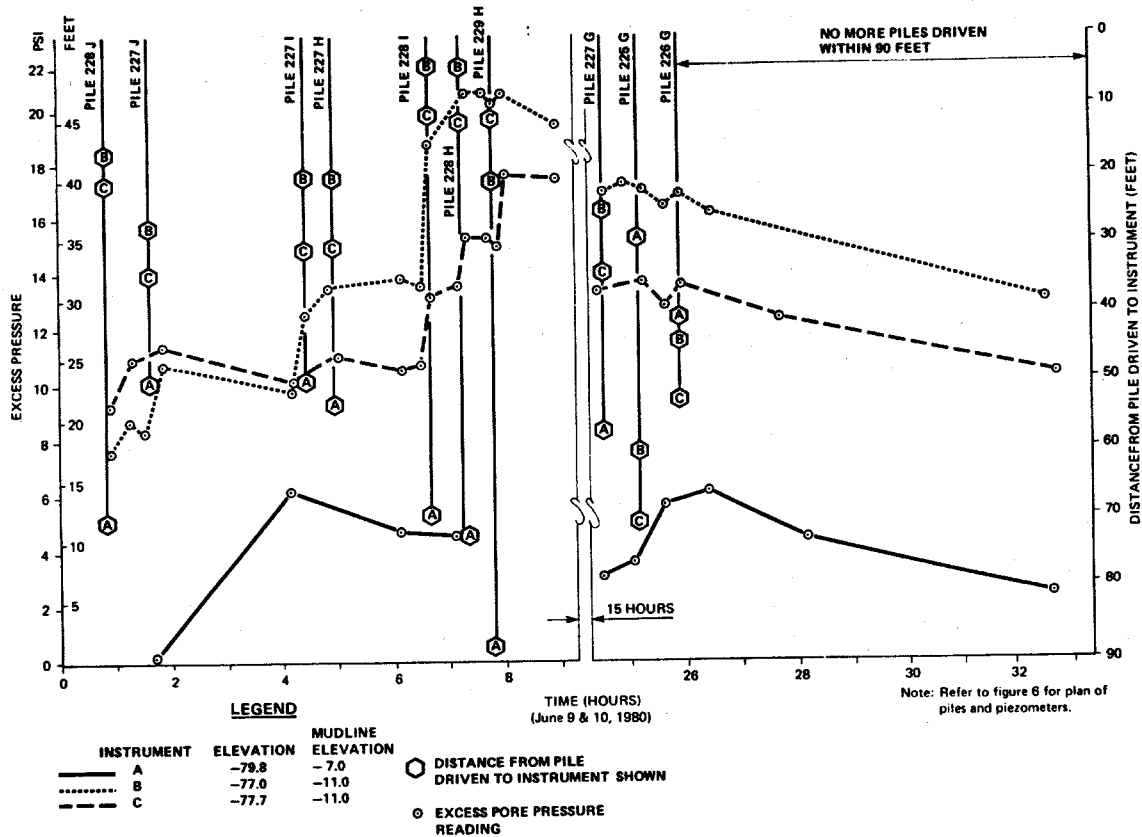
Figure 9. Pore pressures during pile driving (phase C).
