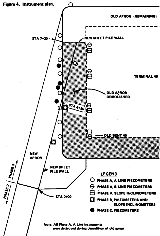
Figure 4. Instrument plan.
